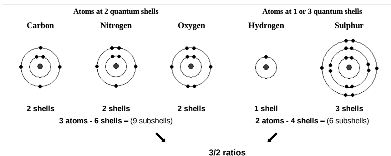
Figure 11: Differentiation of the 5 atoms constituting the 20 proteinogenic amino acids into 2 sets of 3 and 2 atoms according to the parity of their number of electron shells.
