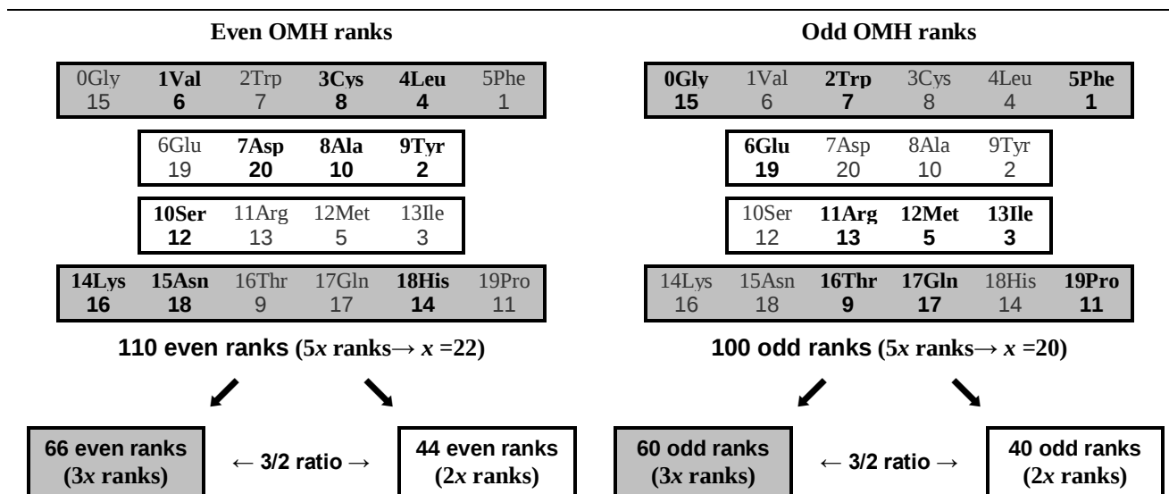
Figure 18: According of the rank parities: OMH index ranks distribution in exact 3/2 ratio into two external and internal sets of AAs.
