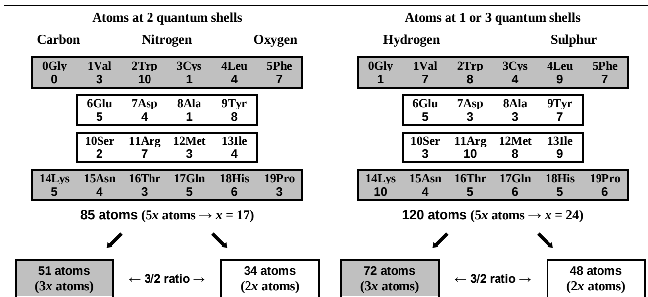
Figure 12: Atom counting inside radical of each proteinogenic amino acid. Distribution in 3/2 ratio regarding AAs numbering and number parity of electron shells.
