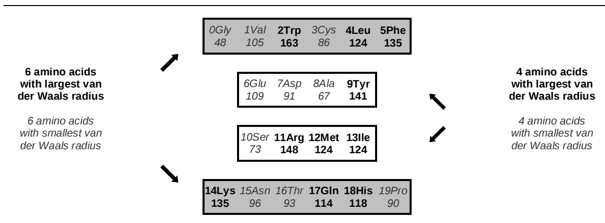
Figure 27: Van der Waals radius index distribution in 3/2 ratio according to AAs internal and external numbering.
