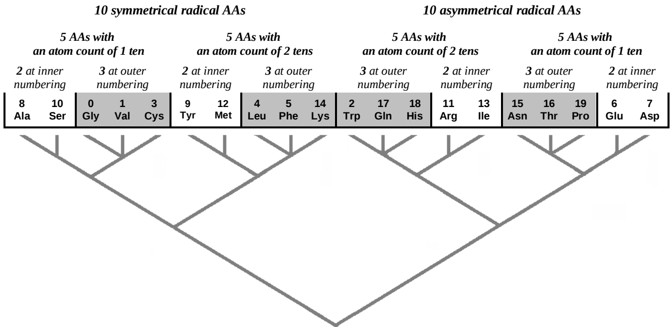
Figure 44: Fractal distribution of amino acids according to two physico-chemical criteria and to one numbering criterion (derived from the physico-chemical properties of nucleobases). Appearance of the final 3/2 ratio in this fractal configuration of the genetic code.
