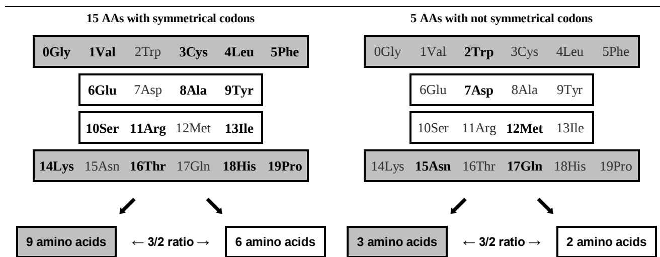
Figure 50: Distribution in 3/2 ratios of the two AA sets at symmetrical codons (same 1 st and 3 rd identical nucleobases) or at not symmetrical codons according to predefined numbering zones.
