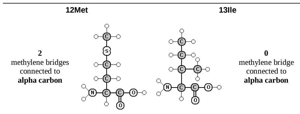
Figure 14: CH 2 groups (methylene bridges) differentiation.
