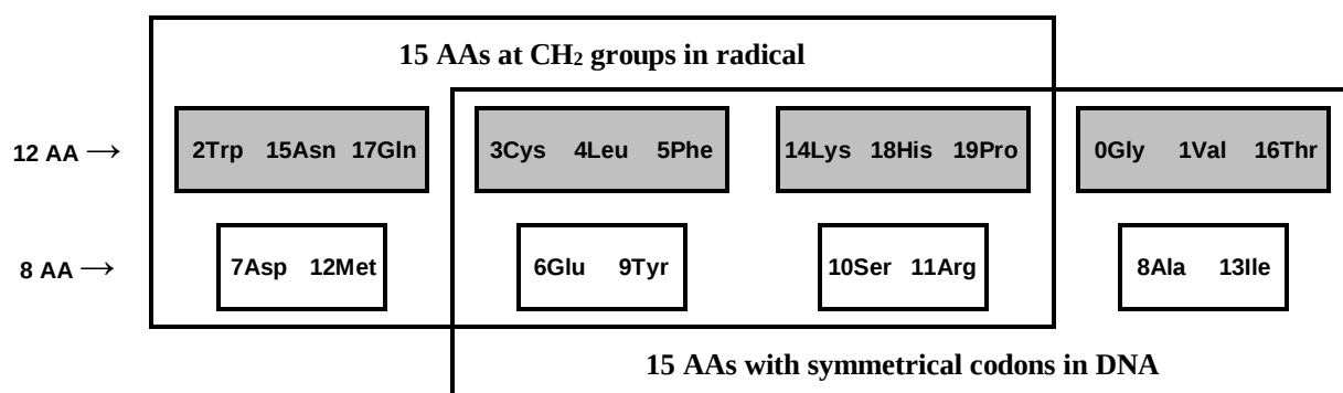
Figure 53: Criterion symbiosis of nature coding and molecular structural and transcending also with numbering concept. See Fig. 50, Fig 51 and 52 also.
