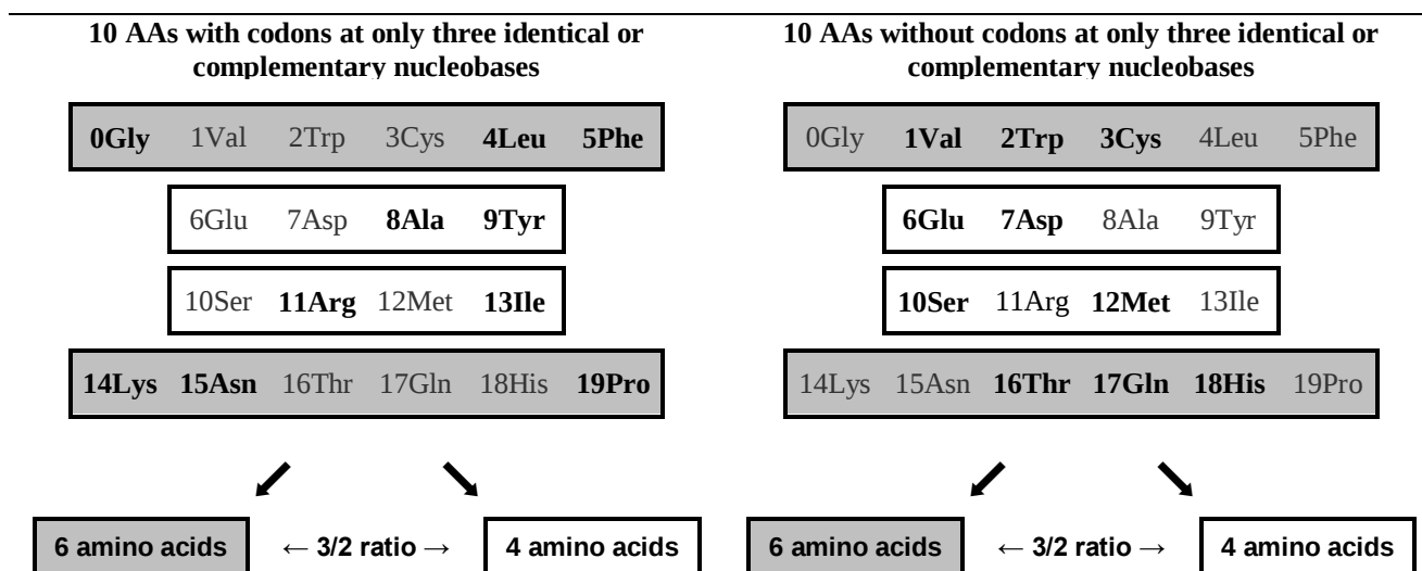
Figure 47: Distribution in perfect 3/2 ratios in the two predefined numbering zones of the two AA sets with or without codons at only three identical or complementary nucleobases. See Figure 46 also about genetic code.
