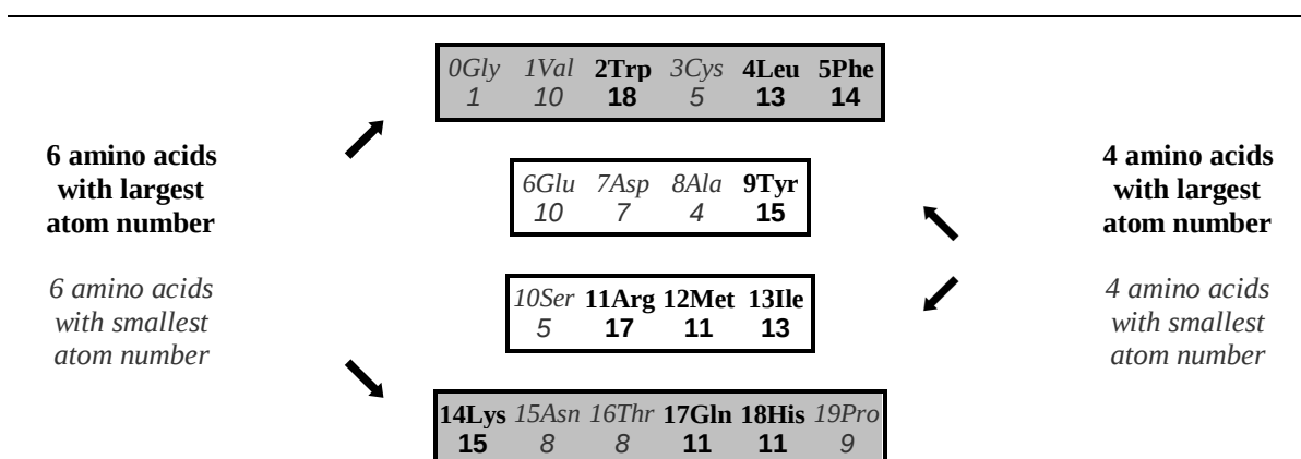
Figure 28: Largest and smallest atom number AAs distribution in 3/2 ratio according to internal and external numbering. See Fig. 27 also.
