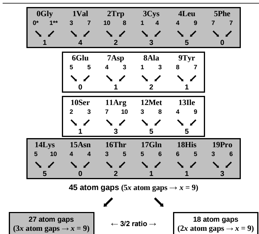
Figure 13: In absolute values: atom gap counting regarding number parity of electron shells. * C,N and O. ** H and S. See Fig. 12 also.
