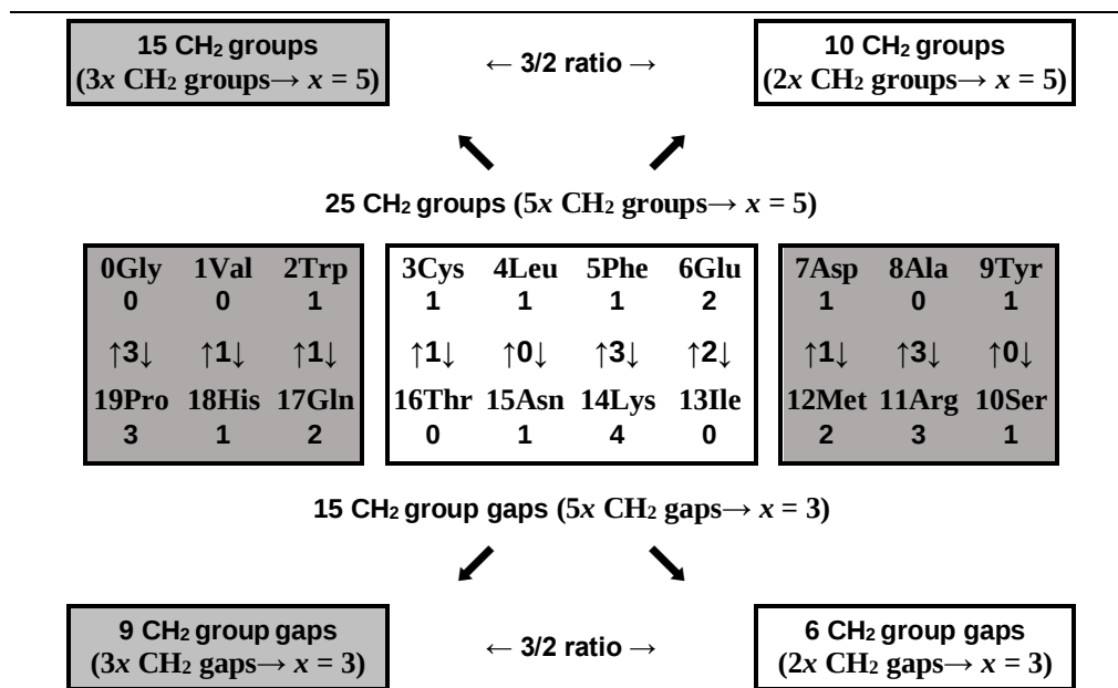
Figure 57: CH 2 groups counting in two new symmetrical numbering zones of 12 versus 8 entities.
