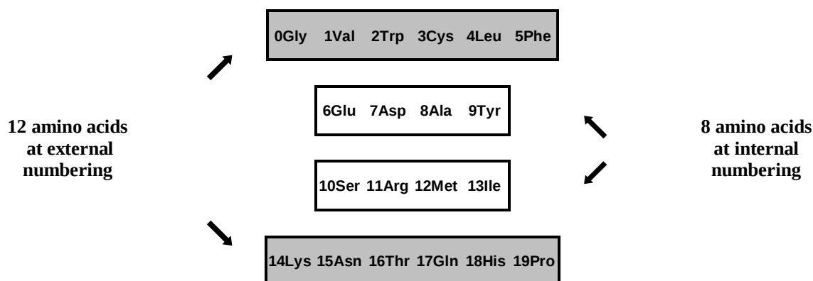
Figure 6: Conventional representation of 20 proteinogenic amino acids numbering in symmetry graphics.
