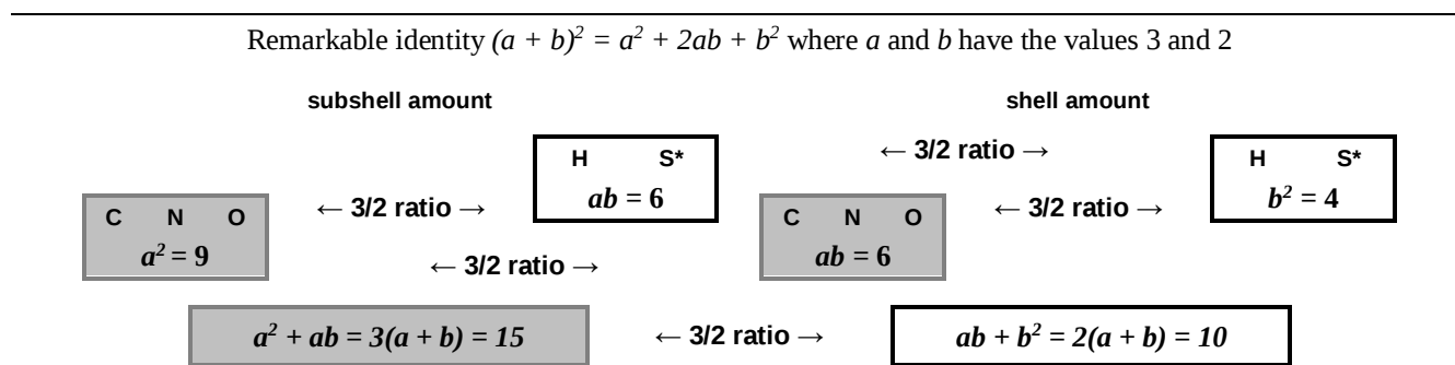
Figure A4: Remarkable identity revealed in the count of subshells and quantum shells of the five elements H, C, N, O and S (*P in DNA). See Fig. A3. See Fig. 56 chapter 10.1 for comparison.
