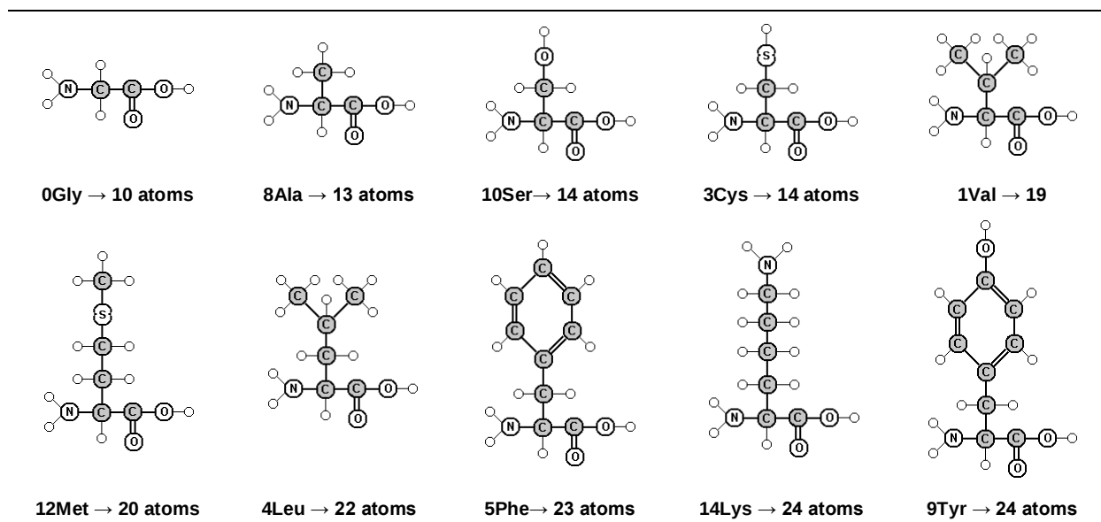
Figure 39: The ten amino acids with symmetrical radical: 5 AAs at atom count from 10 to 19 and 5 AAs from 20 to 29.
