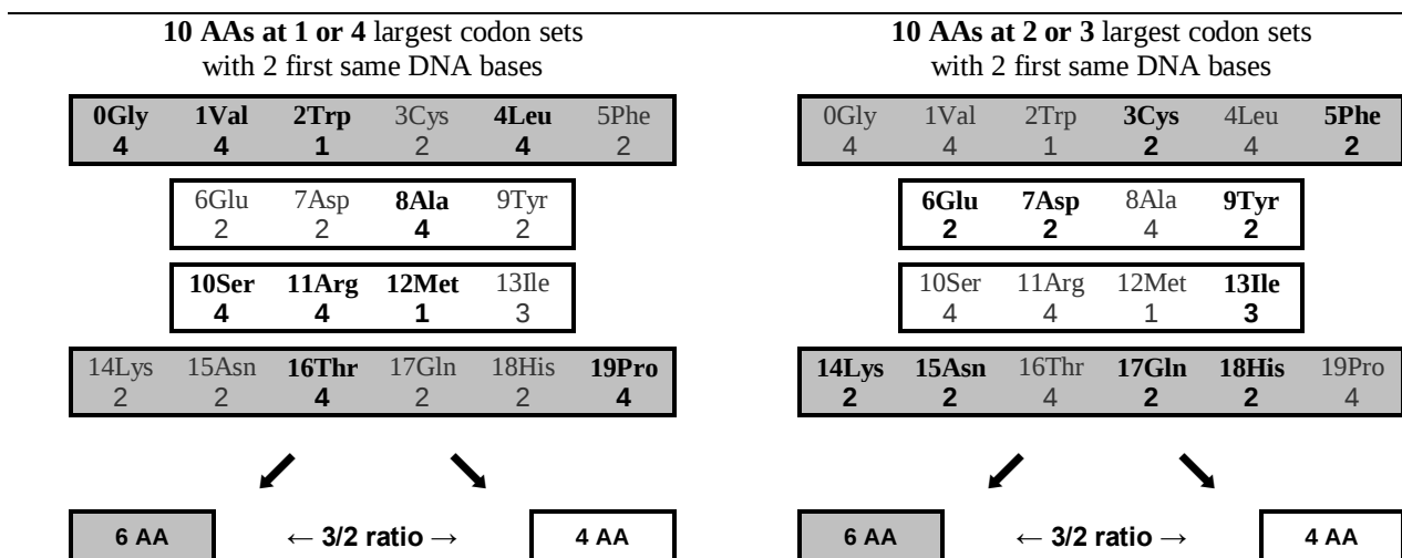
Figure 45: AA distribution in perfect 3/2 ratios in the two predefined numbering zones according to greatest codon number set. See Fig. 19 also about lighter genetic code.
