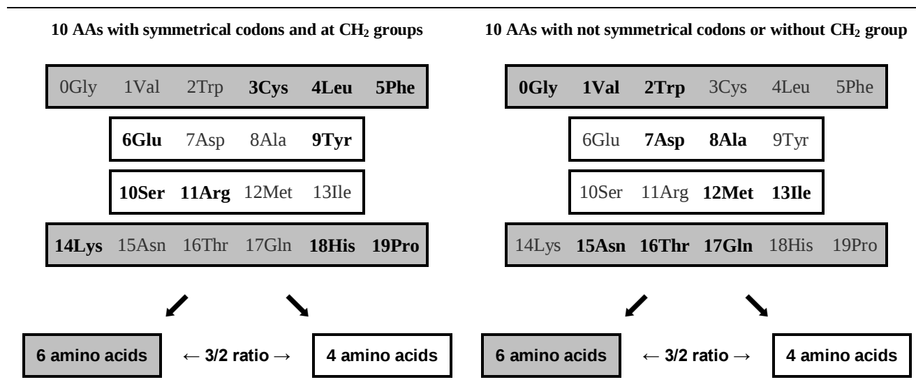
Figure 54: The two sets of 10 AAs generated from CH 2 group concept and symmetrical coding concept.
