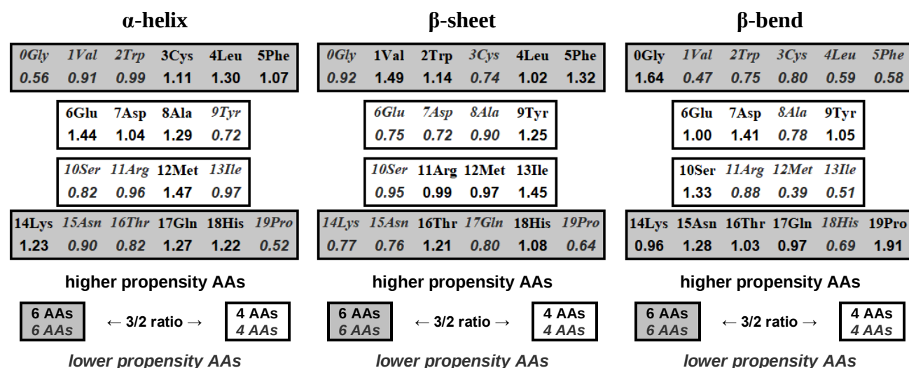
Figure 29: Garnier-Osguthorpe-Robson scales index distribution in 3/2 ratio according to AAs internal and external numbering. See Fig. 22 and 23 also.
