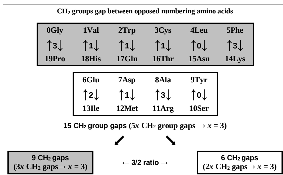
Figure 16: CH 2 groups gaps between opposed numbering amino acids. See Fig 15 also.
