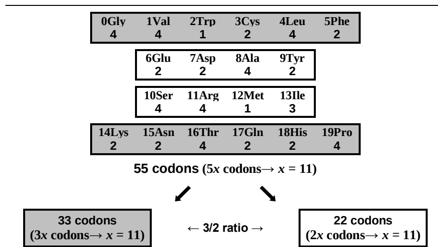
Figure 20: Codon number in largest codon sets with 2 first same DNA bases.
