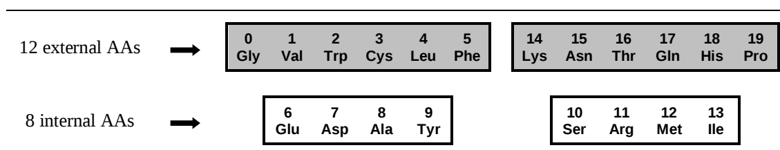
Figure 5: Since them numbering, symmetrical break-up of the 20 AAs into two sets of 2 times 6 versus 2 times 4 entities.
