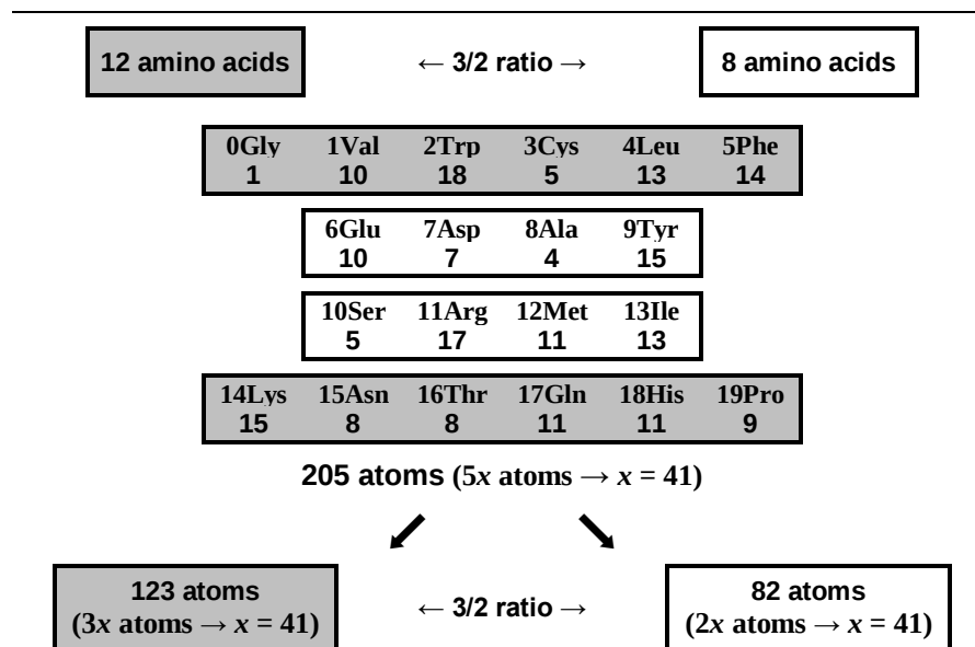
Figure 10: Atom counting inside radical of each proteinogenic amino acid. Distribution in 3/2 ratio regarding AA numbering areas.
