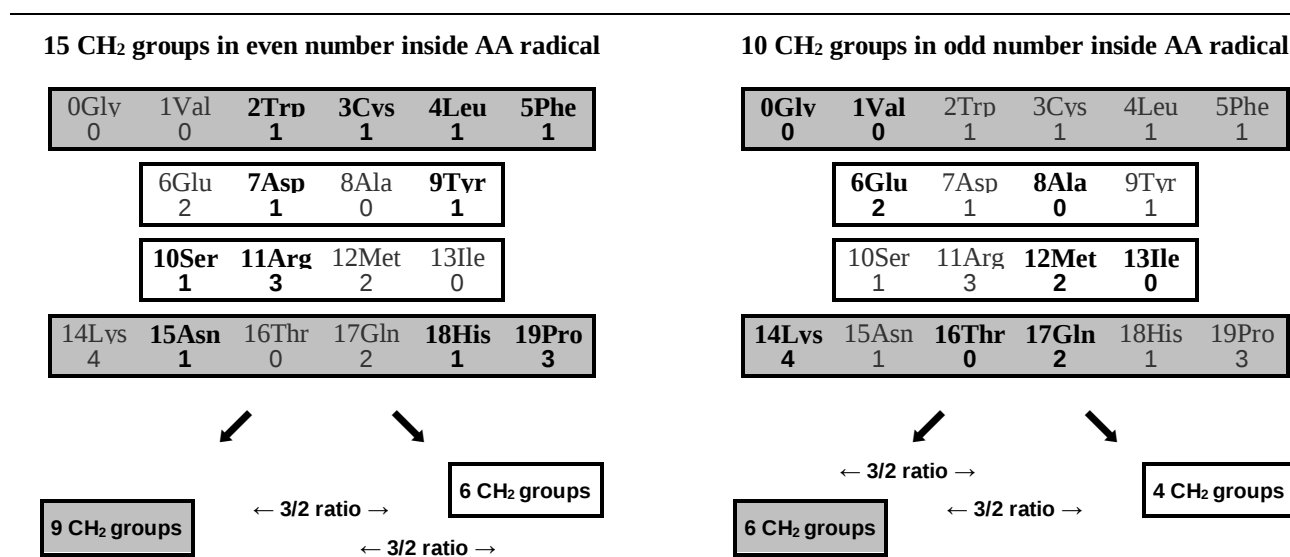
Figure 55: Distribution of the 25 CH 2 groups in various and interconnected 3/2 ratios according to the parity of their number in the radicals and of the two predefined numbering zones.
