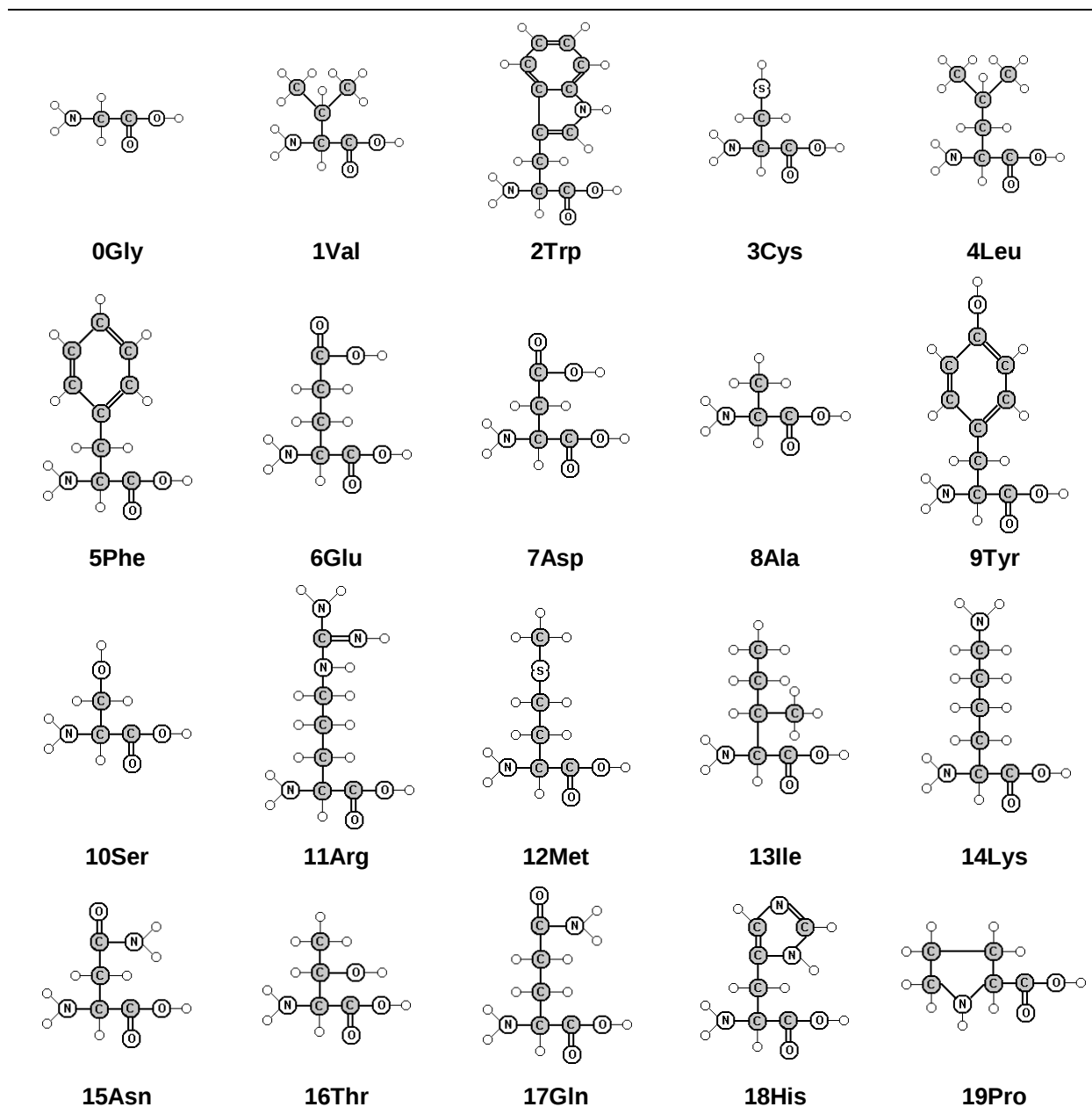
Figure 8: Molecular description of the 20 proteinogenic AAs in the order of their numbering (in an unconventional graphic design which is inspired by S. Petoukhov papers [1-2]).
