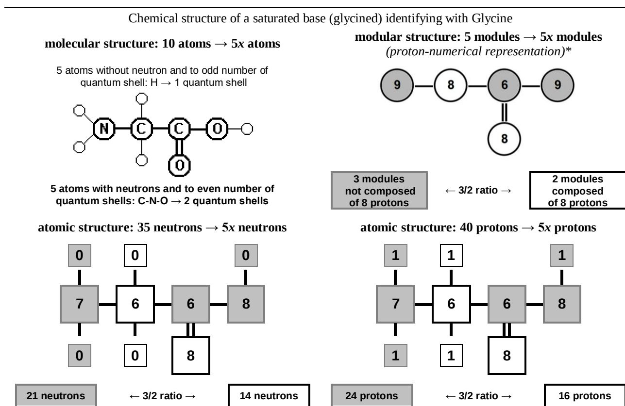
Figure A1: Chemical, modular and atomic structure of a saturated base identified with the amino acid Glycine: 5 modules, 10 atoms, 40 protons and 35 neutrons. See also Fig. A2. * inspired representation from Sergey Petoukhov [1 and 2].
