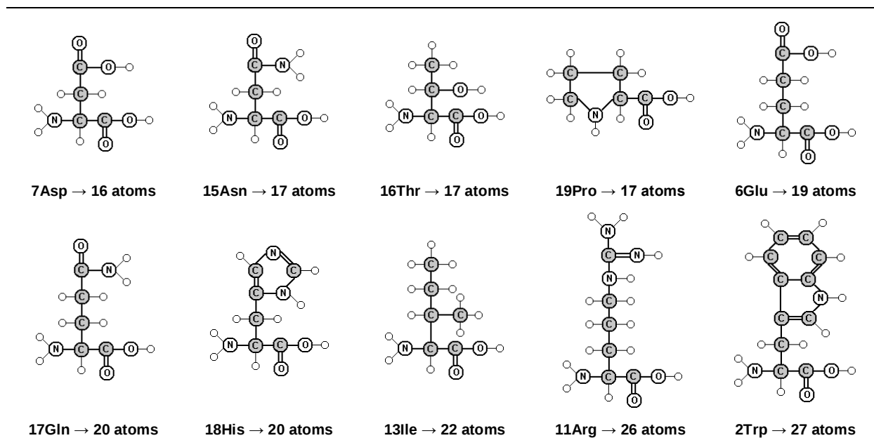
Figure 40: The ten amino acids with asymmetrical radical: 5 AAs at atom count from 10 to 19 and 5 AAs from 20 to 29.
