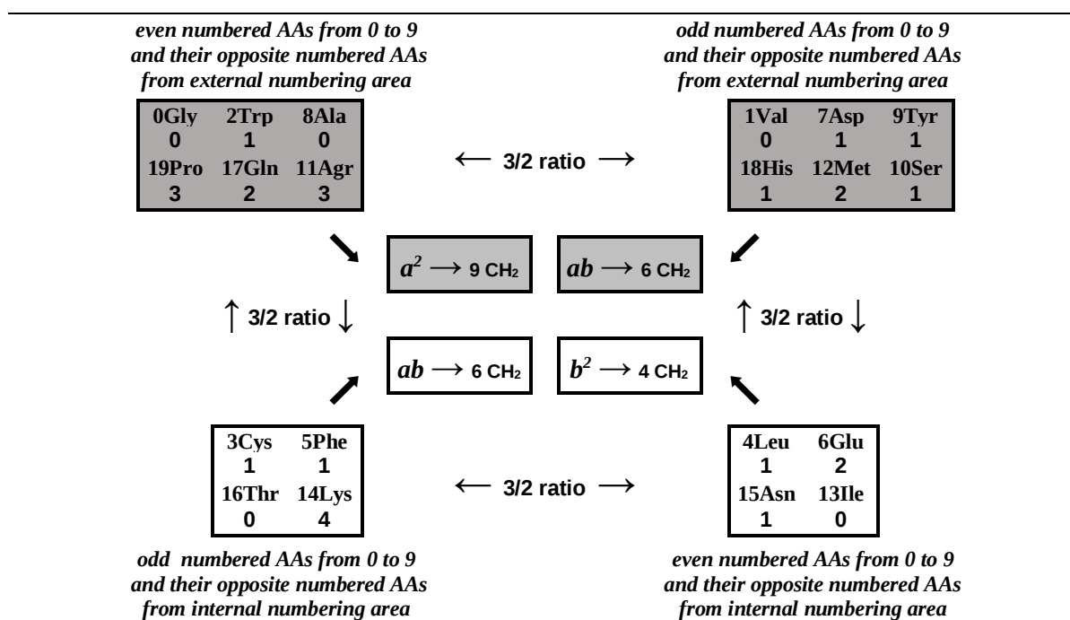
Figure 58: Organisation in remarkable identity of 25 CH 2 groups according to the AAs numbering parity and new numbering areas.
