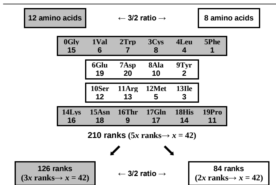
Figure 17: OMH index ranks distribution in exact 3/2 ratio into two external and internal sets of AAs.
