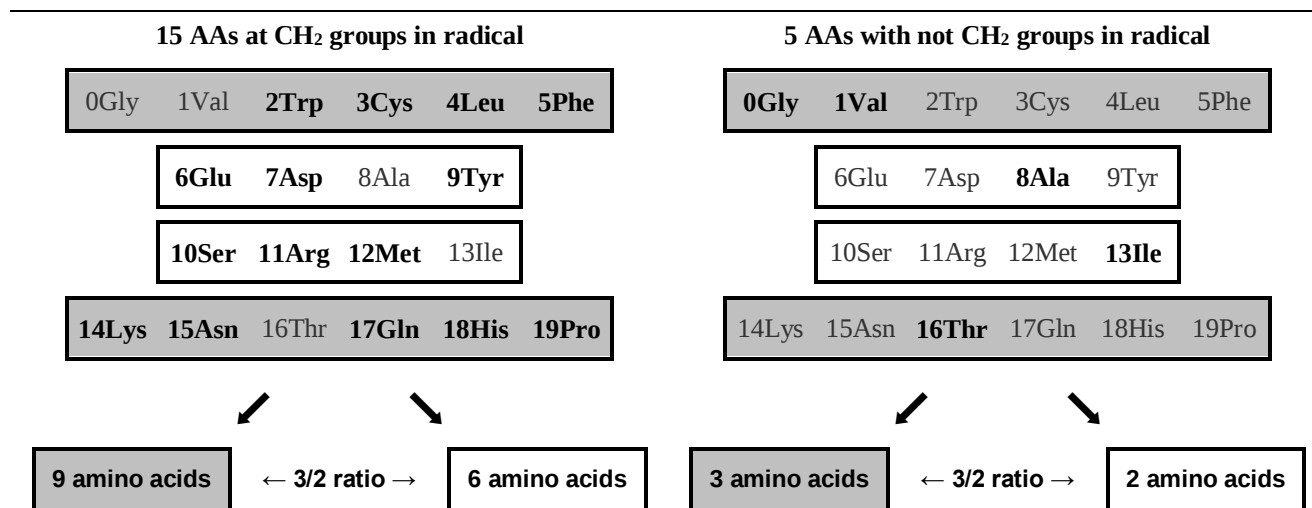
Figure 51: Distribution in 3/2 ratios of the two AA sets with CH 2 groups in radical or without CH 2 groups according to predefined numbering zones. See Figure 7 Chapter 3.1 and Figure 14 Chapter 4.3 also.
