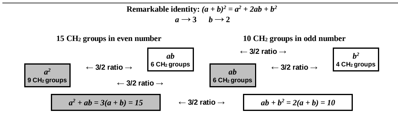
Figure 56: Remarkable identity revealed in the count of CH 2 groups in even number or in odd number and according to numbering areas. See Figure 55 also. See Figure A4 in appendix for comparison.
